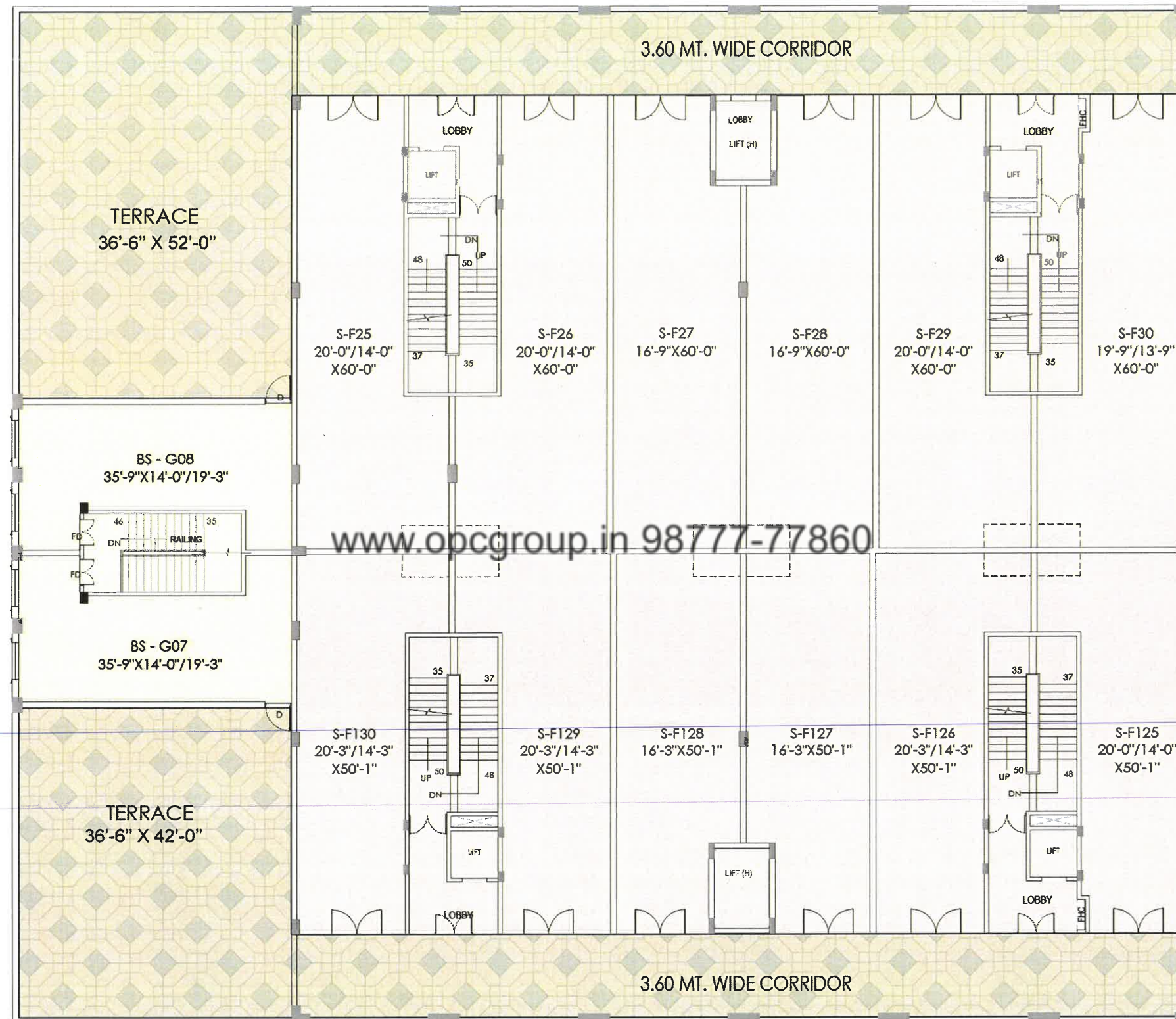
FIRST FLOOR PLAN : BLOCK - B3
