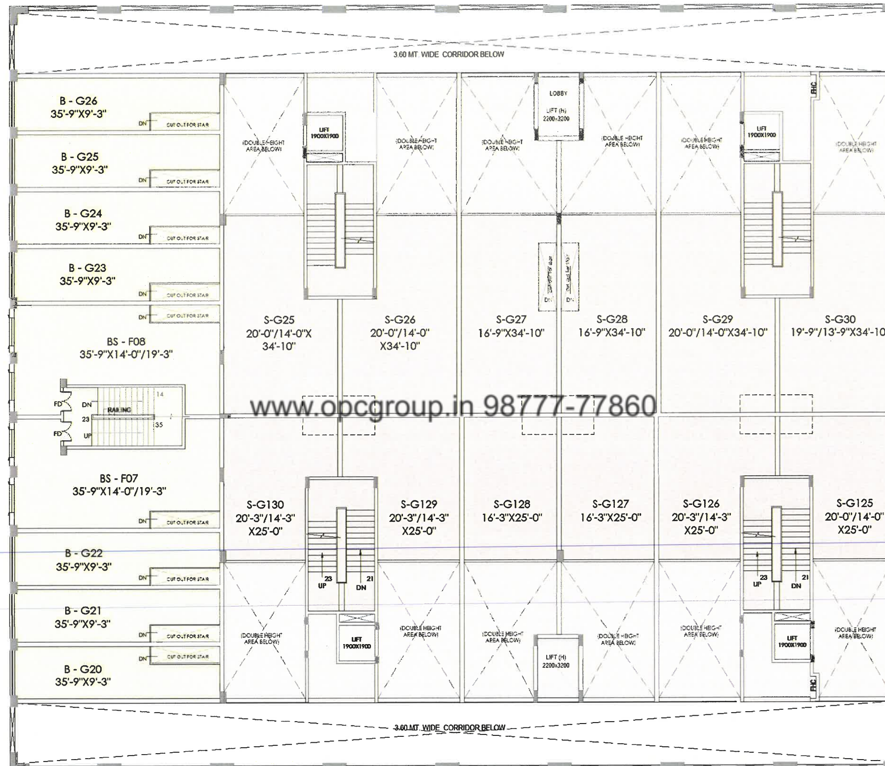
MEZZANINE FLOOR PLAN : BLOCK - B3
