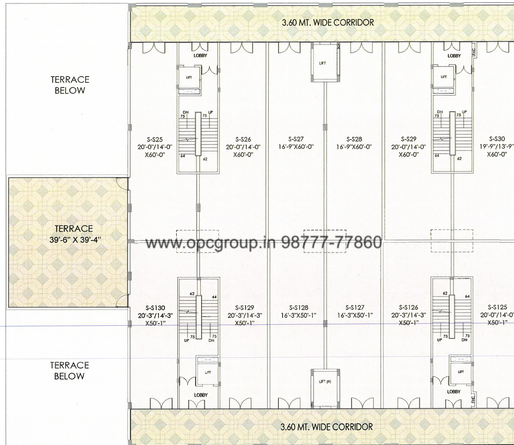
SECOND FLOOR PLAN : BLOCK - B3
