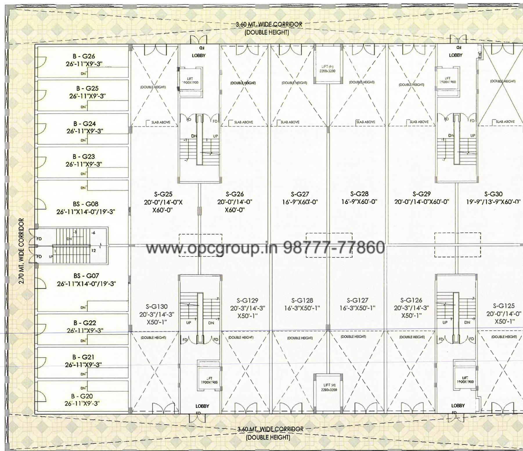
GROUND FLOOR PLAN : BLOCK - B3
